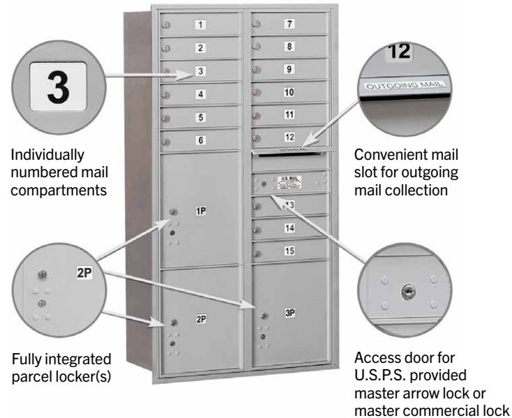
Front view of 3716D-15 Front Loading Recessed Mounted Double Column Unit displayed
